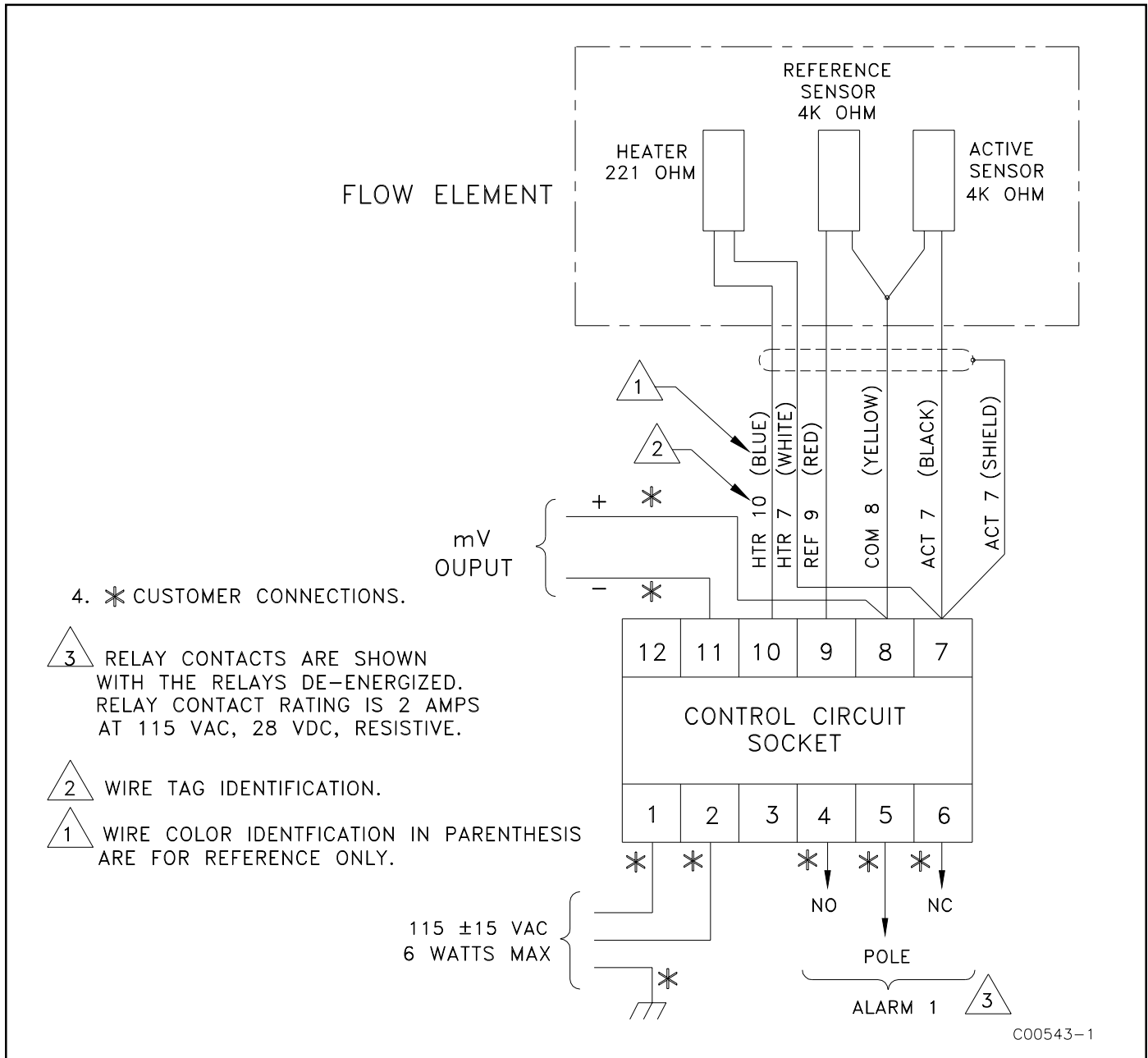
Figure A-2. Wiring Diagram
