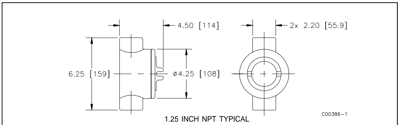
Figure A-3. Optional Remote Type 4 Enclosure
